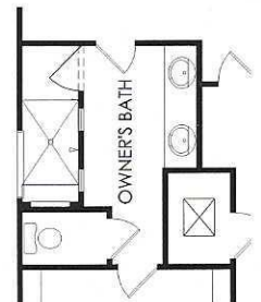
Owner's Bath Layout 6
